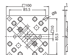
4010-08 Drive bearing on base plate including screws and nuts
