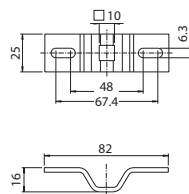
4010-04 Awning drive bearing for awnings with 48 mm semicircle
